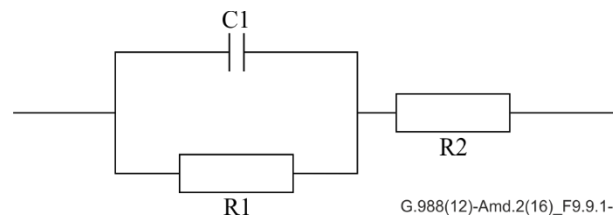
Figure 9.9.1-1 – Impedance model for POTS UNI
