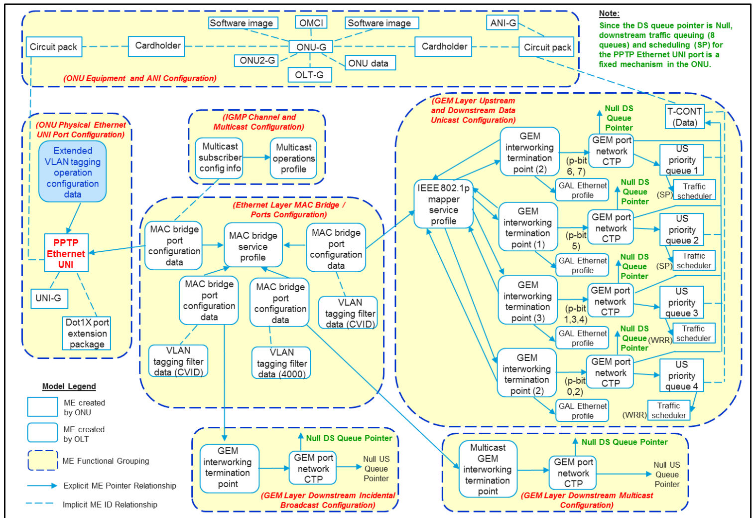
Figure 13 – Physical Ethernet UNI Data Service ME Model
