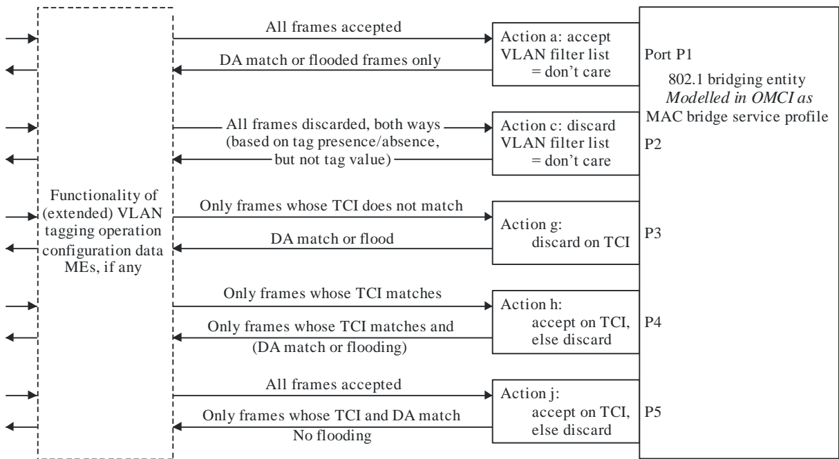
Figure 7 - Forwarding Behavior
